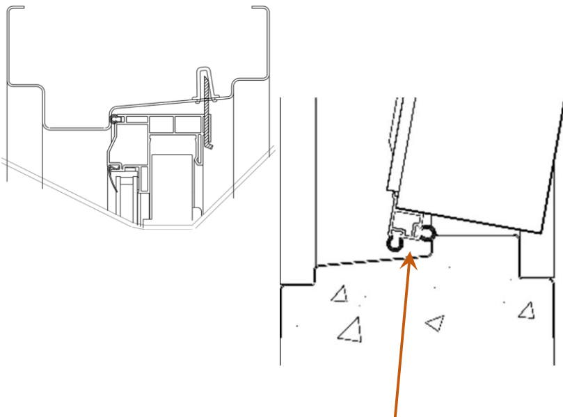
Sill Adapter VPro4 Window
